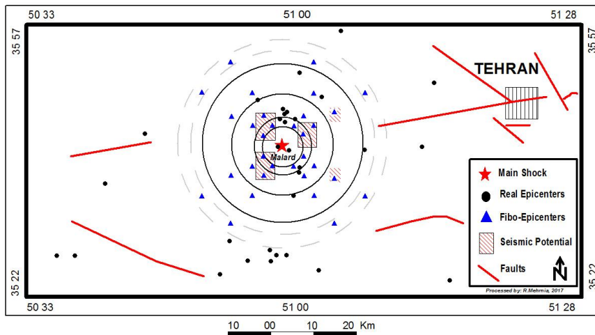
Figure 4. A Fractal separation in random - regular Fibonacci sequences in Malard seismic events (20 Dec. 2017)
