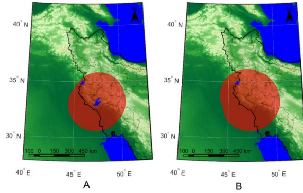
Fig. 1. Integrated alarm maps, the gray regions are alarm areas, the star sign is Sarpol-e Zahab earthquake epicenter, A) The alarm investigation points at t_{end} in all six modes and union of their circles, B) intersection of the alarm areas at t_{end}
