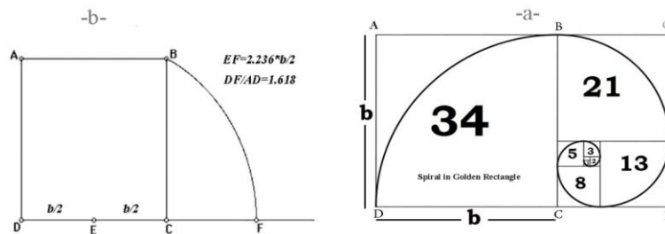
Fig. 1. Spiral function of earthquakes based on a golden rectangular distribution.
