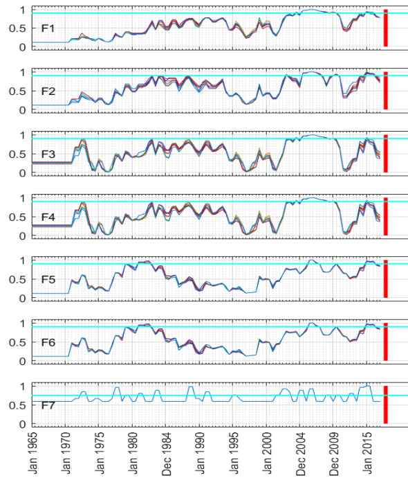
Fig. 2. The value of of the M8 algorithm functions over time for the joint investigation points and \tilde{N}_1 = 4, \tilde{N}_2 = 3 (time of the target earthquake is shown using a thick vertical line)
