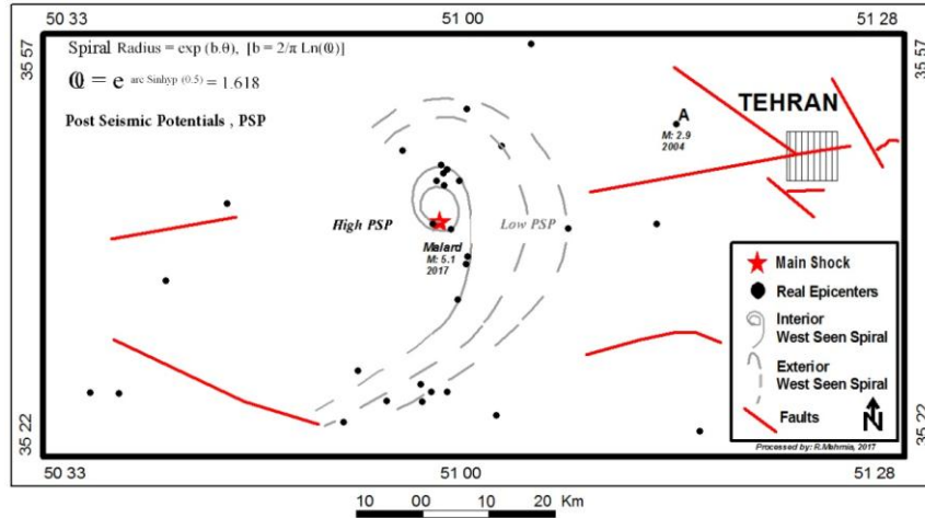
Fig. 3, Spiral distribution of Malard earthquakes (Ref. Database: IIEES, 1964-2017)
