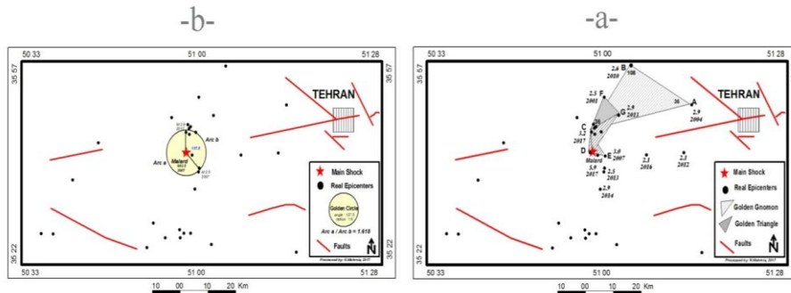
Fig. 2, a) two kinds of golden triangles (ordinary and gnomons) in Malard seismic pattern. b) A symmetric golden circle with approximate radius =1.6 near Malard main shock region.
